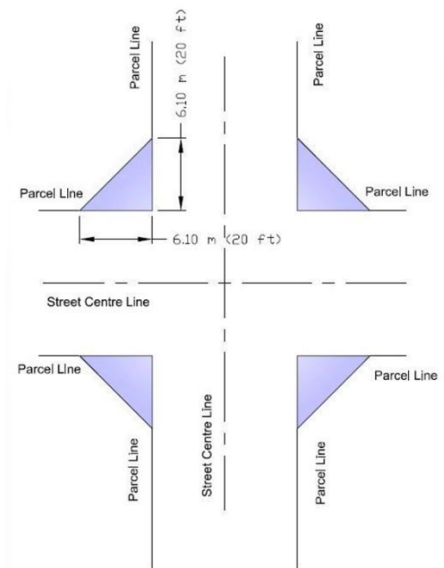
FIGURE 7-1 ILLUSTRATION OF SIGHT TRIANGLE
